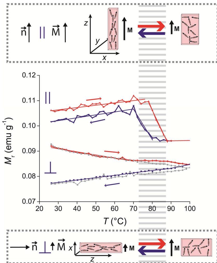
Figure 5. Reversible magnetization change of the OLCE nanocomposite. In a heating-cooling cycle after an initial magnetization (not shown) applied once parallel ( \parallel ) and once perpendicular ( \perp ) to the major susceptibility tensor of the sample, remanence is measured in the magnetization direction. In comparison, the non-oriented LCE nanocomposite is shown (grey symbols, shifted for overlap).
